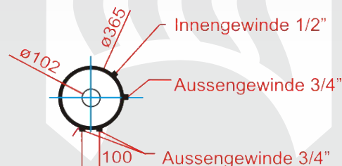
Anschlüsse Z100
